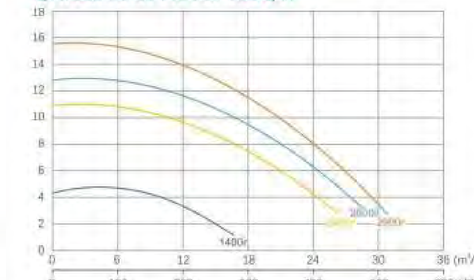
QH.Curve of HLVSP150QW
