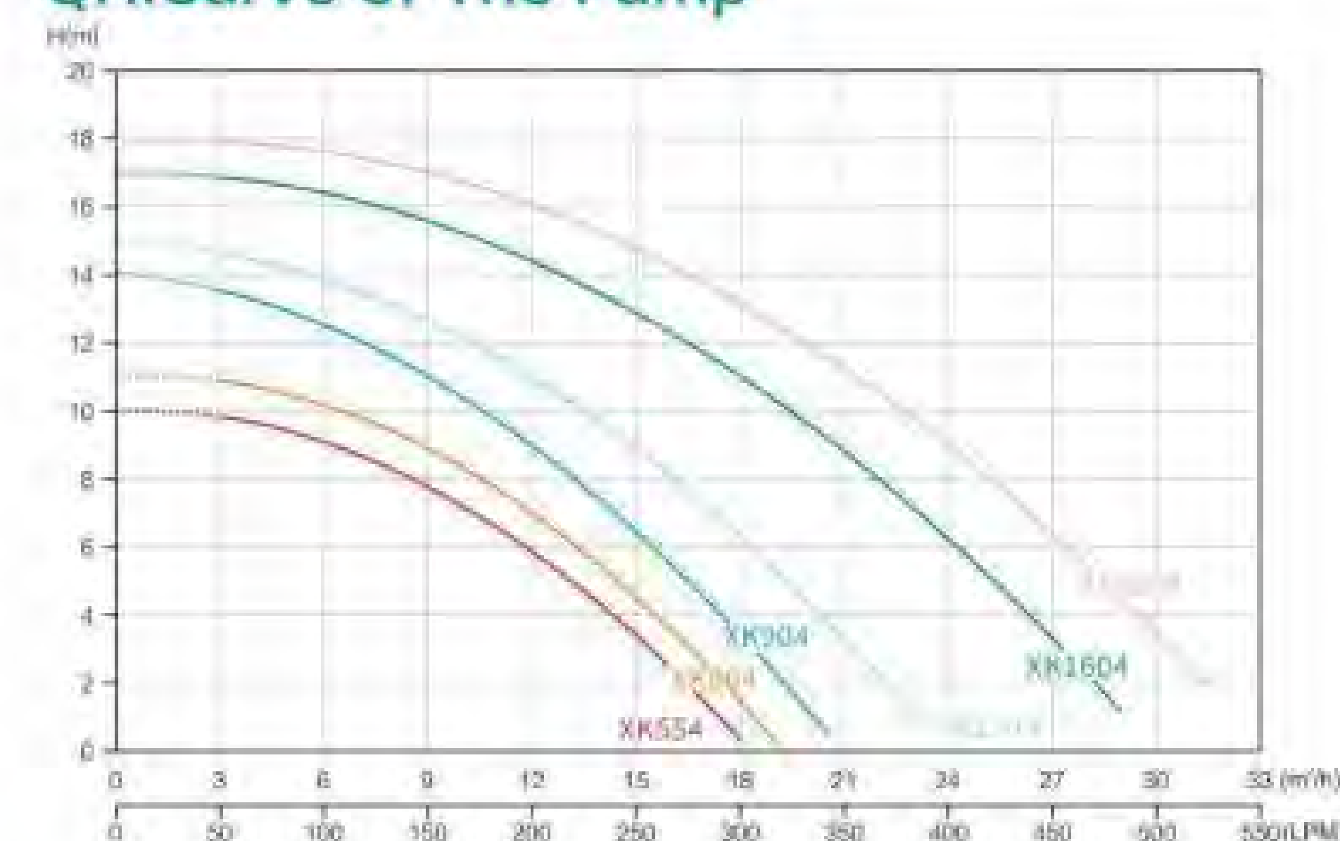
QH.Curve of The Pump
