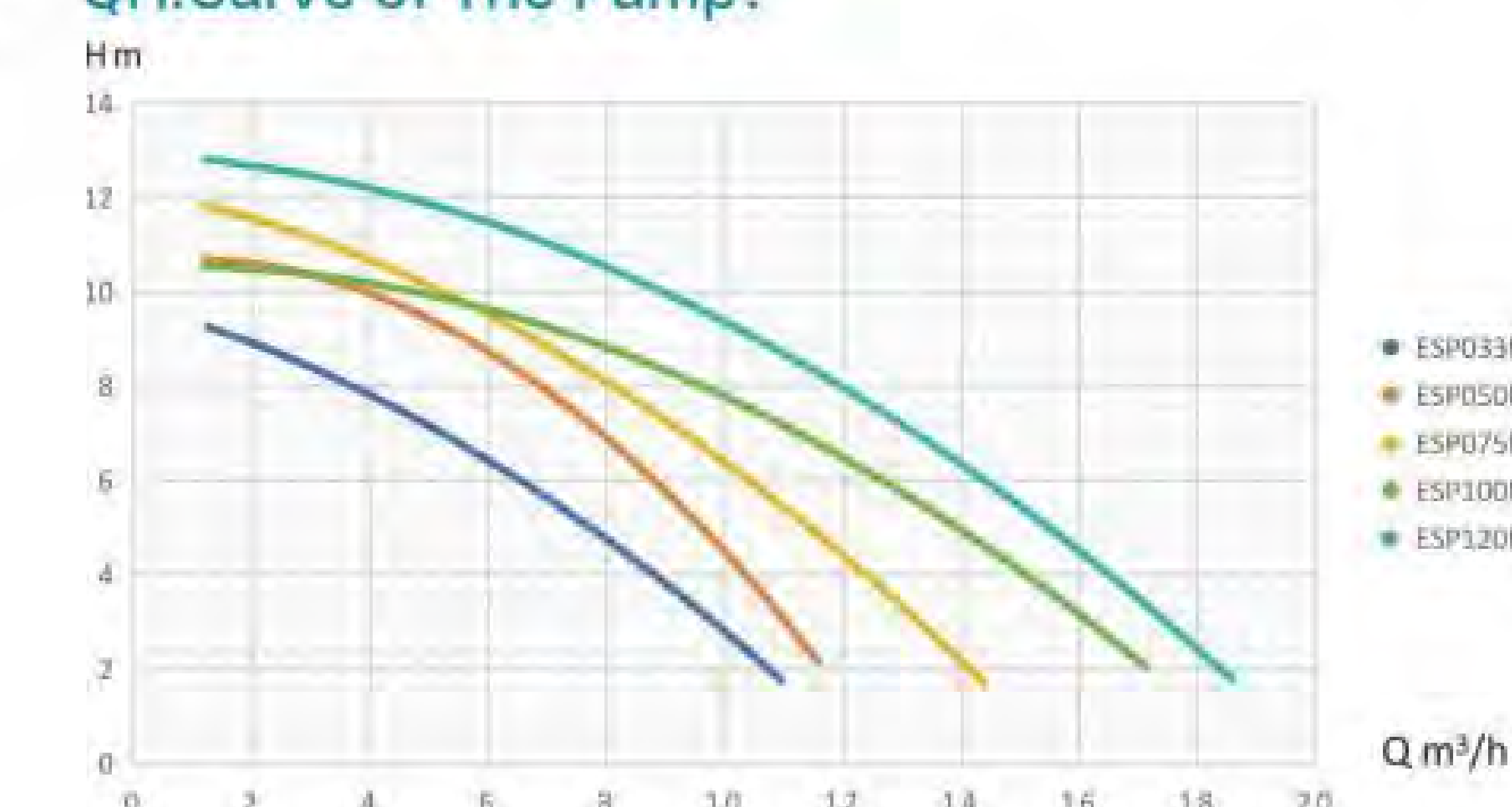
QH.Curve of The Pump:
