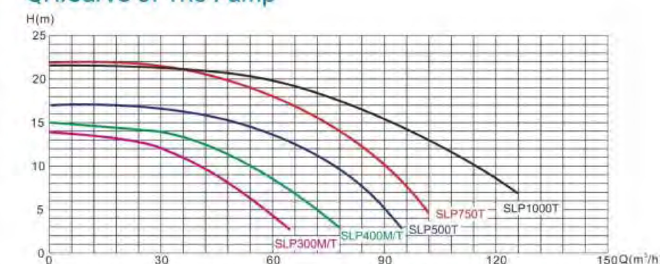
QH.Curve of The Pump
