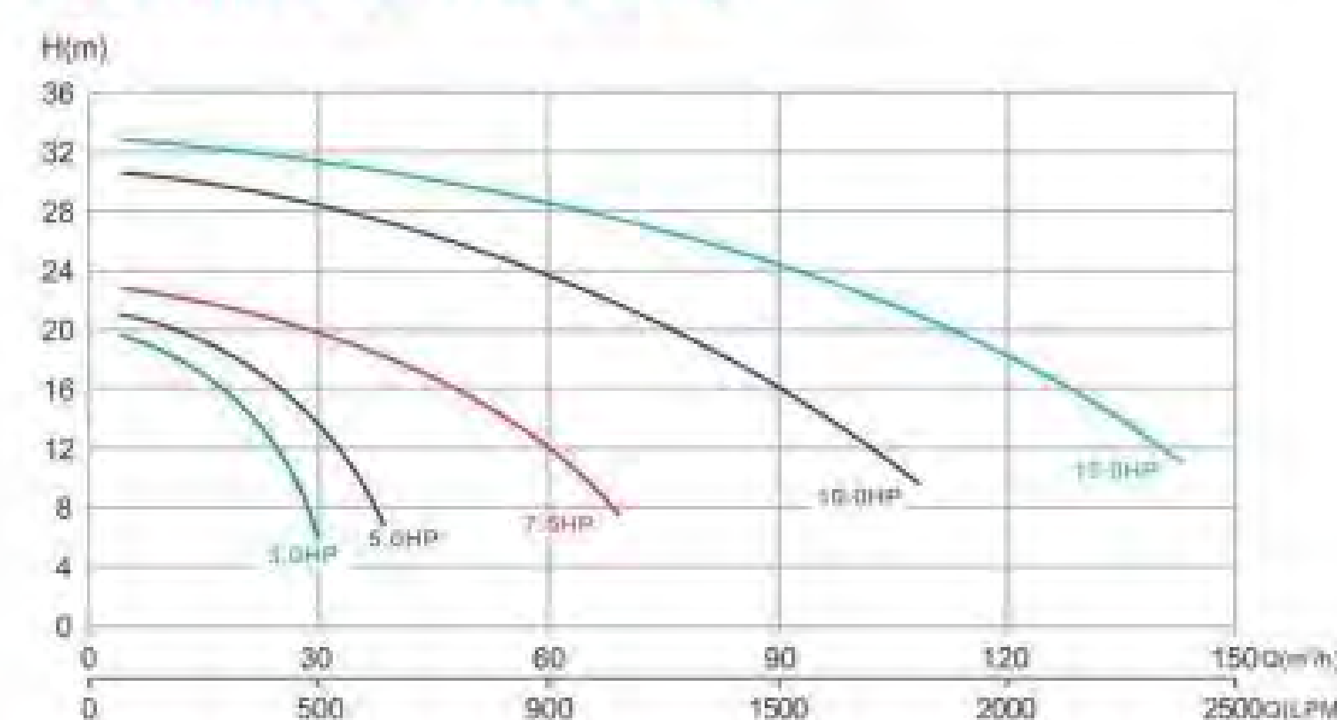
QH.Curve of The Pump
