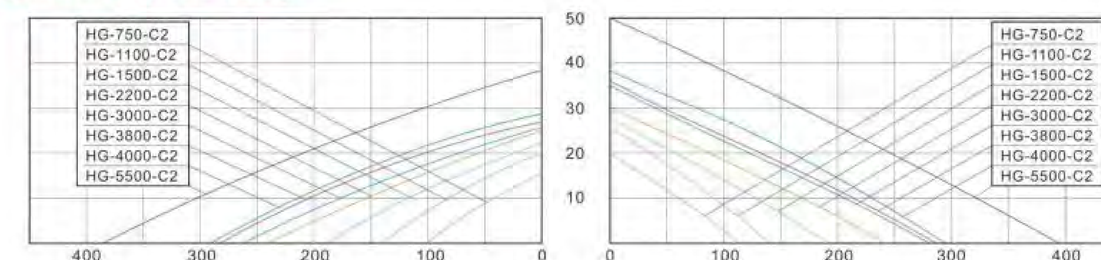
QH.Curve of The Pump
