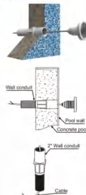
Concrete pool installation with wall conduit:
