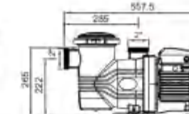
WL-ECP075/100/150
