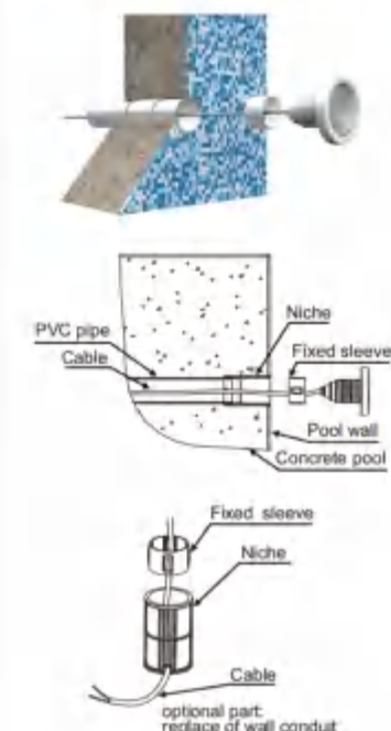
Concrete pool installation to 2"/63mm pipe
