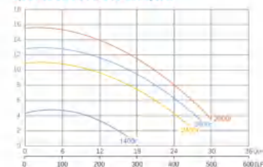
QH.Curve of HLVSP150QWU
