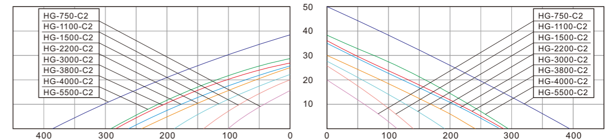
QH.Curve of The Pump
