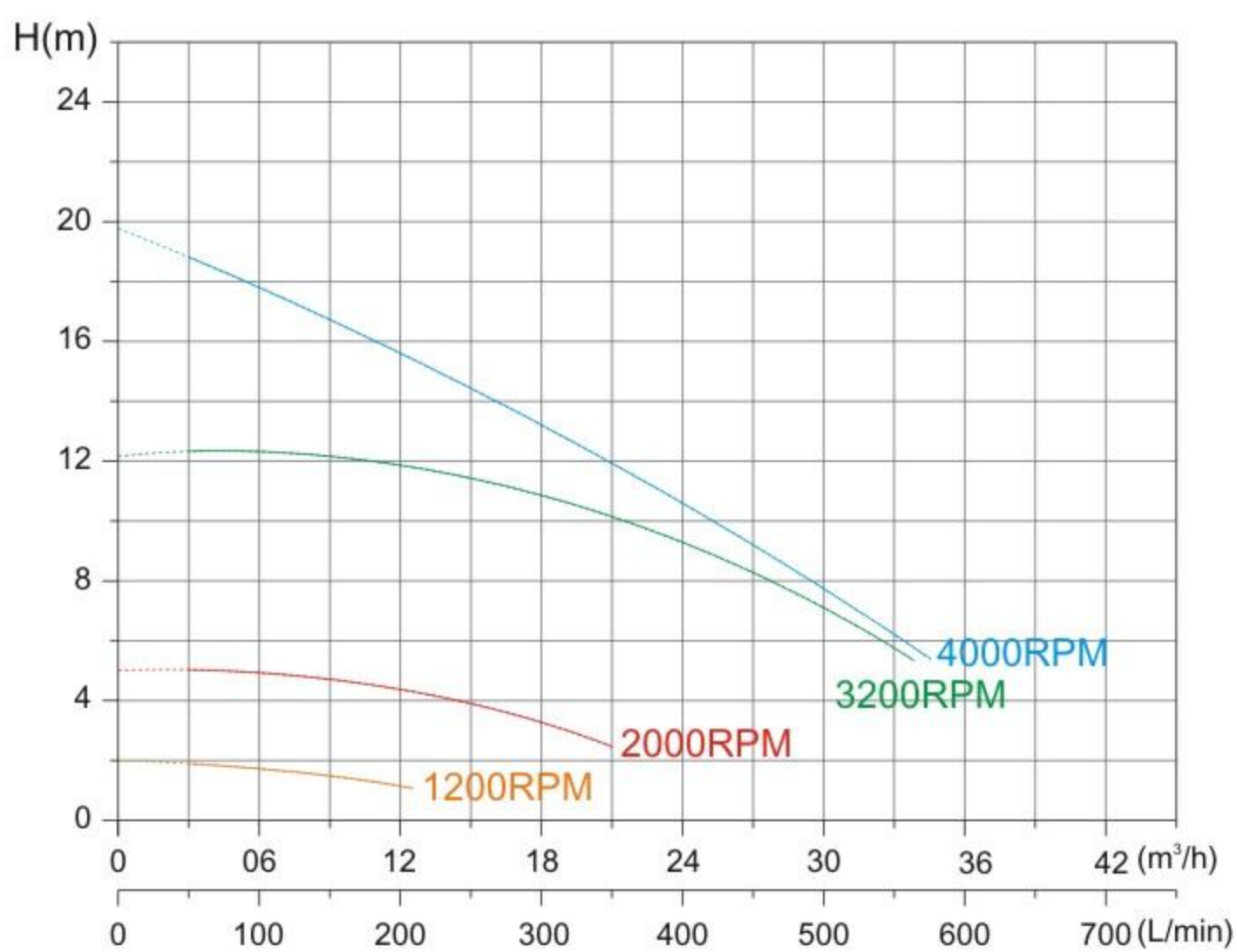
XKP1307BP QH. Curve
