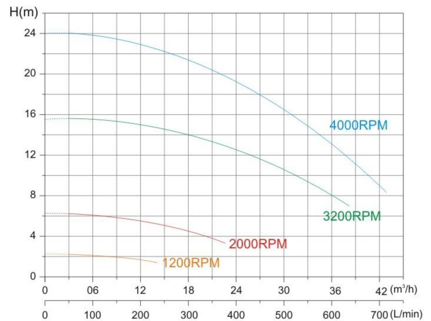
XKP2207BP QH. Curve
