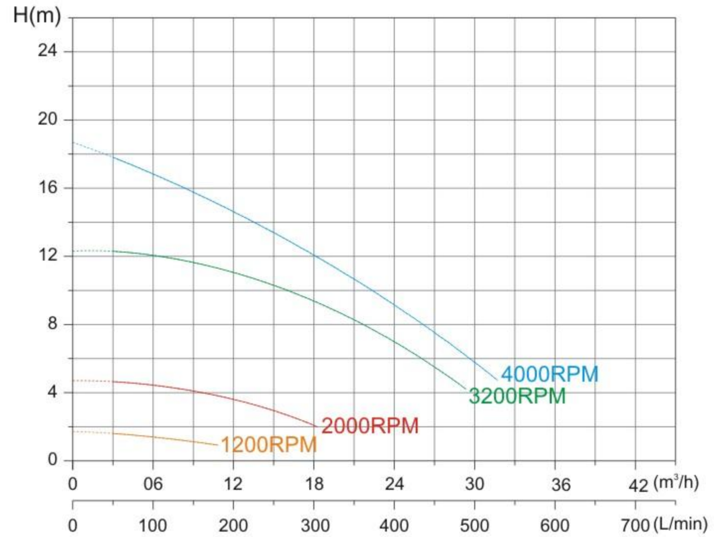
XKP1107BP QH. Curve
