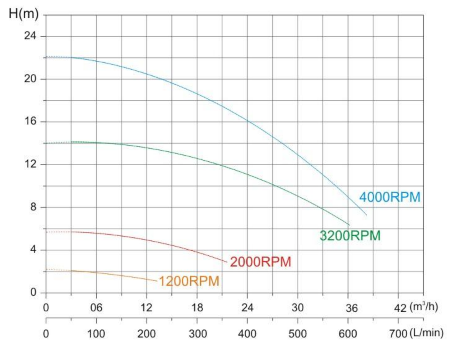
XKP1607BP QH. Curve
