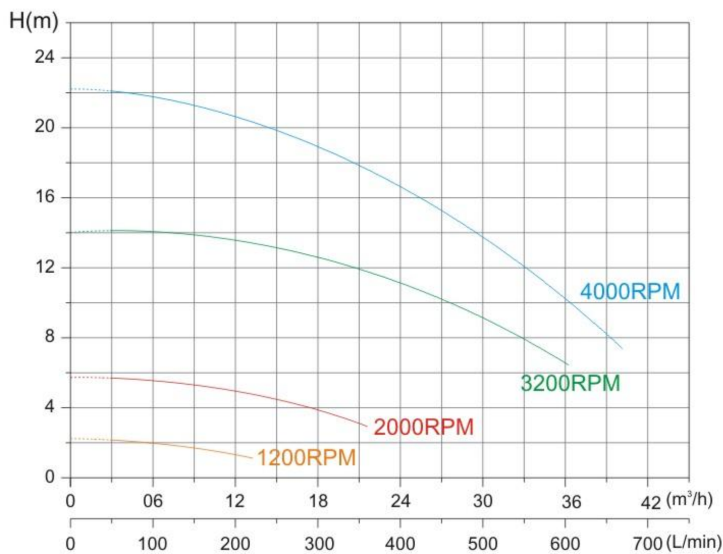
XKP1807BP QH. Curve
