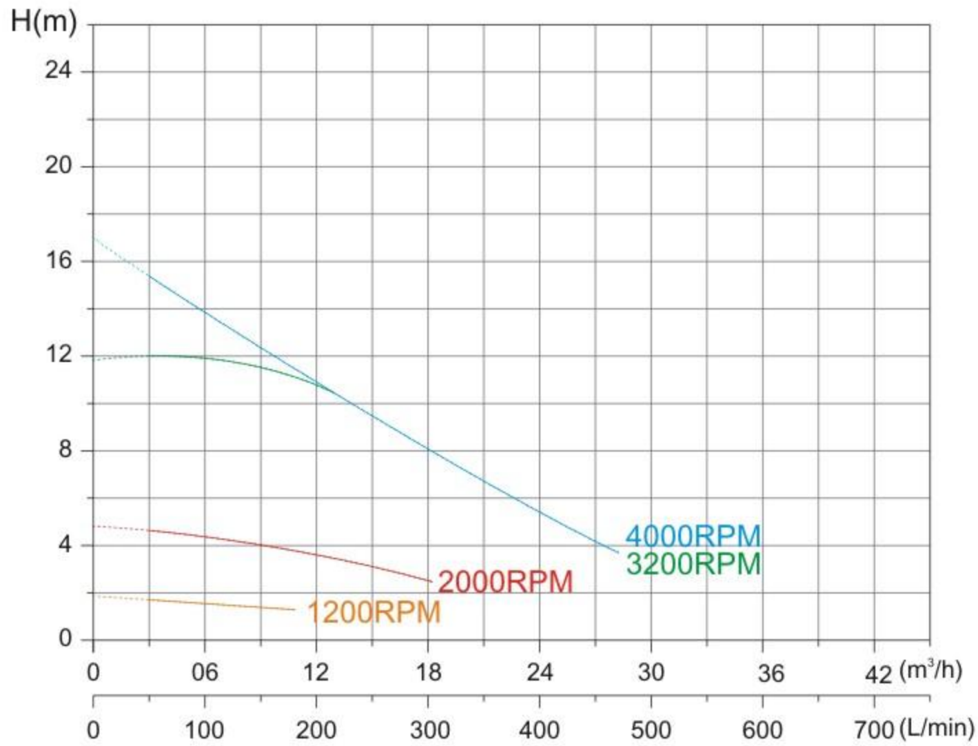
XKP757BP QH. Curve
